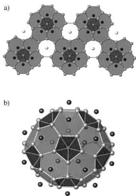
Figure 5. Two observed ways of condensing five face-sharing truncated tetrahedra: a) into ribbons as seen in \text{Li}_{10}\text{Mg}_6\text{Zn}_{31}\text{Al}_3 ; and b) into cages as seen in the Bergman phases found in Li-Mg-Zn-Al systems. [5-7] The truncated tetrahedra are shaded light gray and the pentagonal pyramids created by the condensation of these polyhedra are shaded dark gray.
